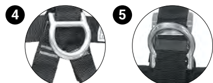
EN 813 Attachment point for sit harness
